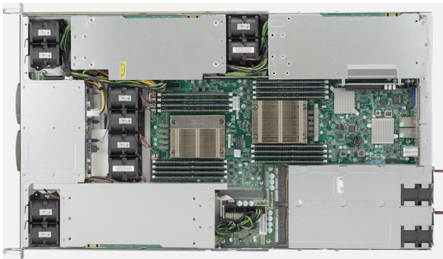
i2090R1 1U GPU server
